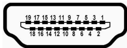
Fig. 4-3: HDMI type A socket
